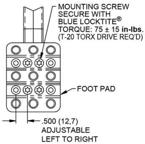
FOOT PAD DETAIL
